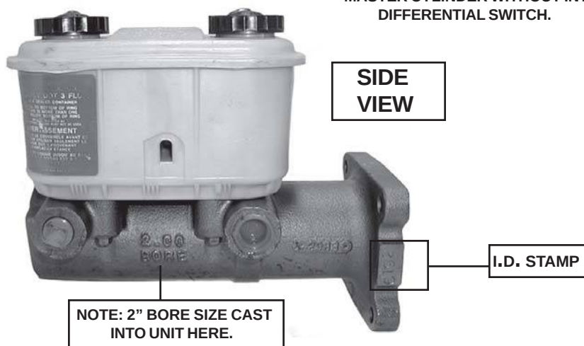
MASTER CYLINDER WITHOUT INTERGRAL DIFFERENTIAL SWITCH.
